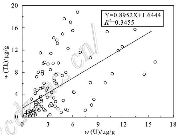
图 2 尕斯库勒盐湖钻孔沉积物 U 和 Th 相关关系图 Fig. 2 Relationship between uranium and thorium in sediments of the drill holes
