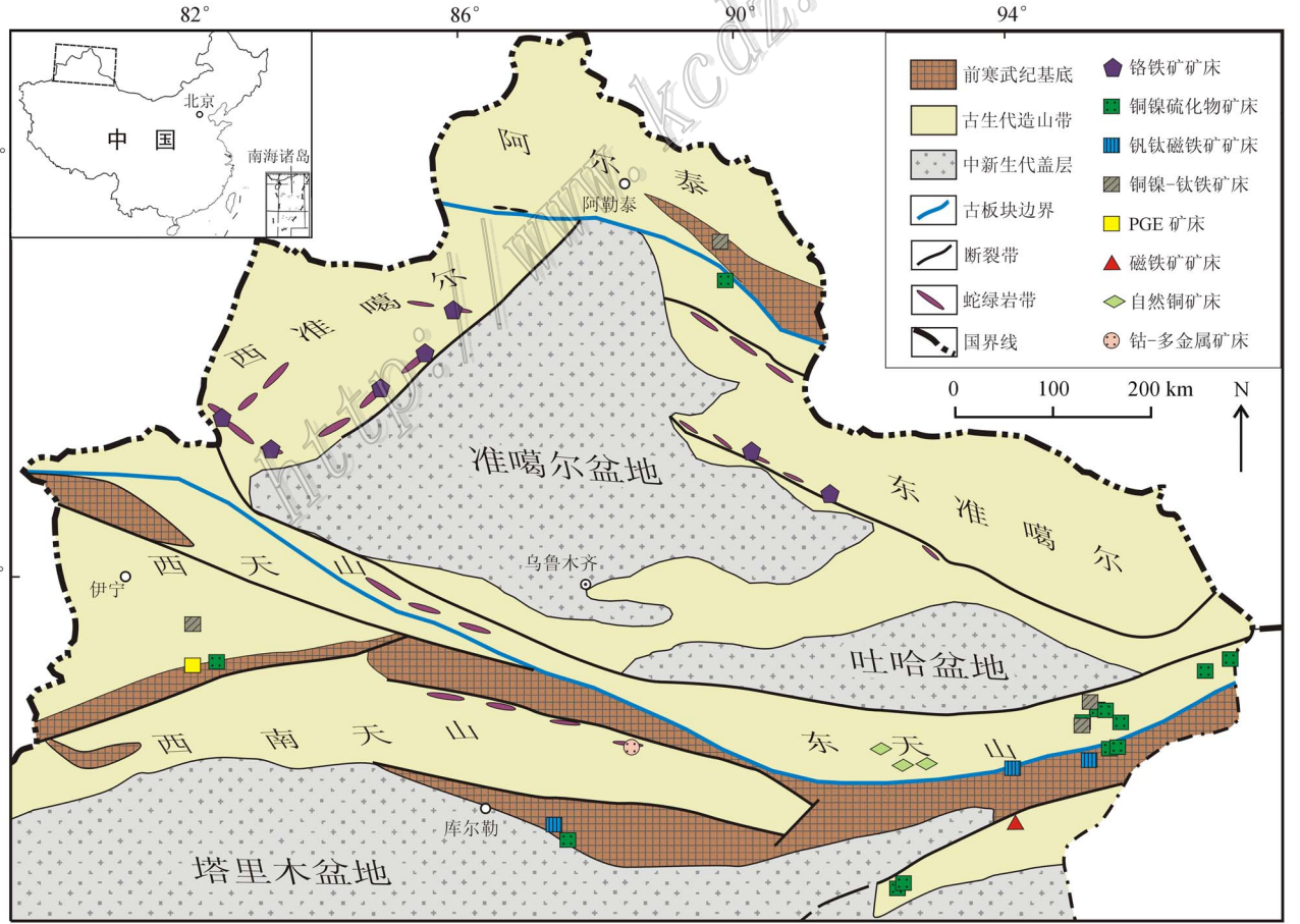
图 1 新疆北部主要幔源岩浆矿床分布图 Fig. 1 The distribution of mantle-derived magmatic deposits in North Xinjiang
