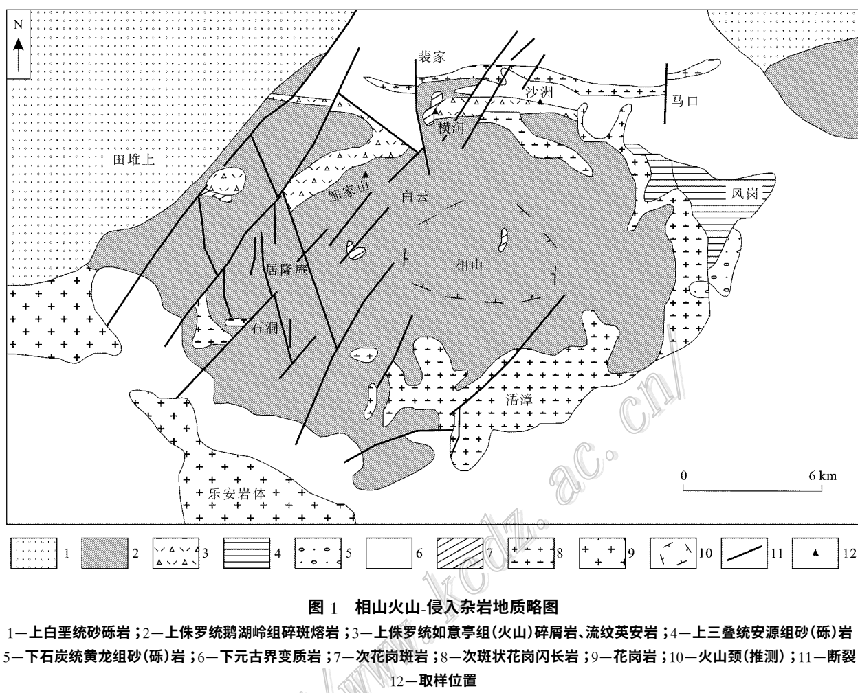
Fig. 1 Geological sketch map of Xiangshan volcanic-intrusive complex
