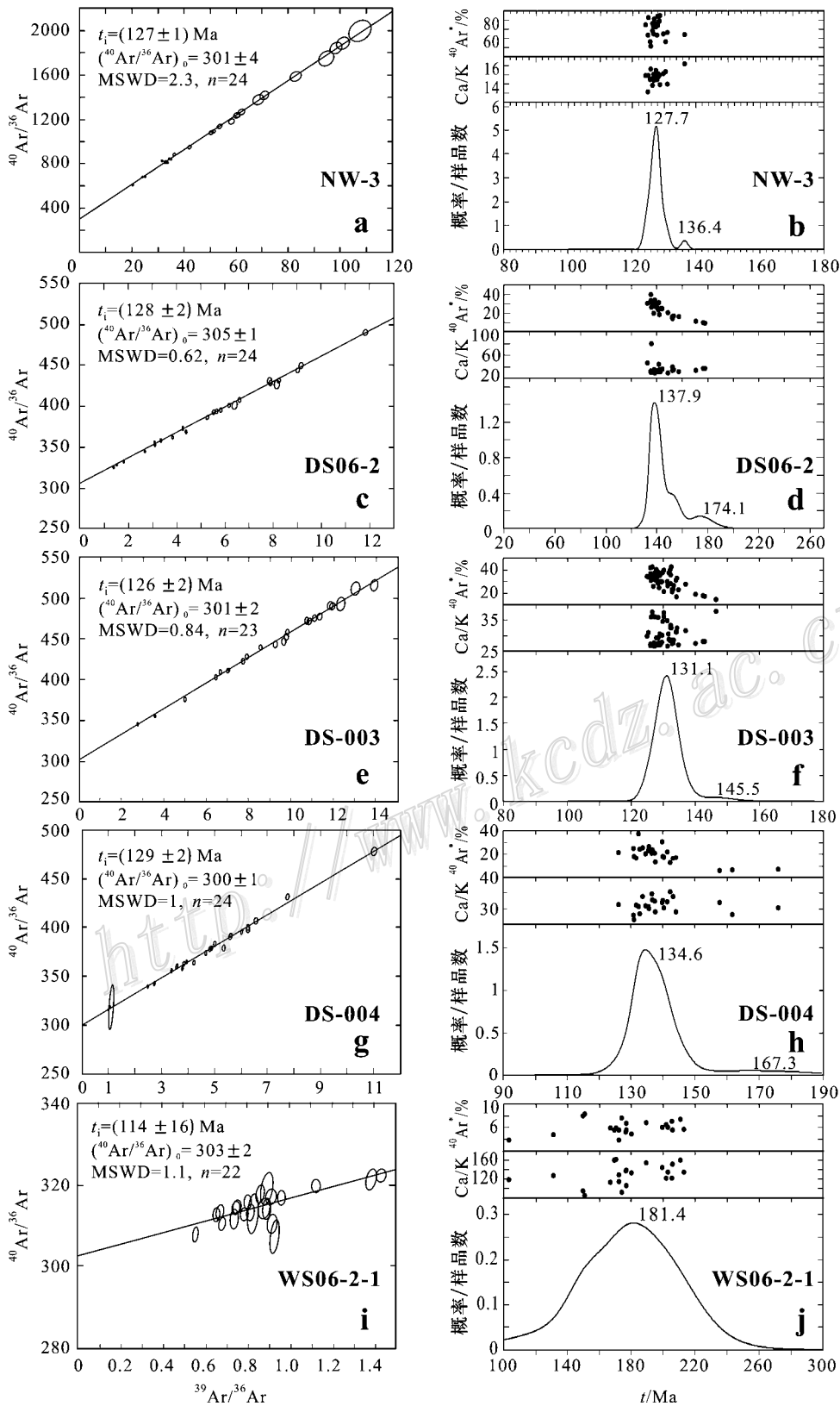
图 2 凹山和东山铁矿床中阳起石和潜火山岩中角闪石 39 Ar- 40 Ar 等时线 (a, c, e, g, i) 和表观年龄 (b, d, f, h, j) 频率分布图 Fig. 2 39 Ar- 40 Ar isochron (a, c, e, g, i) and age-probability diagrams (b, d, f, h, j) of actinolite from Washan and Dongshan iron deposits and hornblende from subvolcanic rocks
