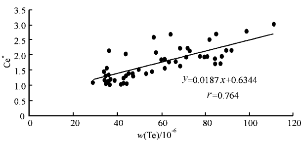
图 3 调查区结壳 \varpi(Te) 元素与 Ce^* 的关系 Fig. 3 Relationship between \varpi(Te) and Ce^* in the crusts from the area
